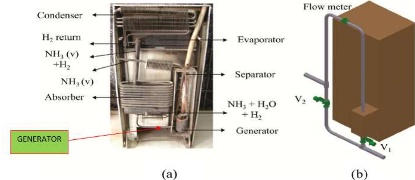
Fig.5: Generator with heating coil
