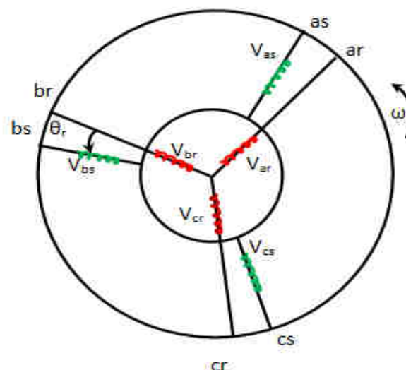
Fig. 5: A 3-phase 4-pole 120 degrees phase apart
