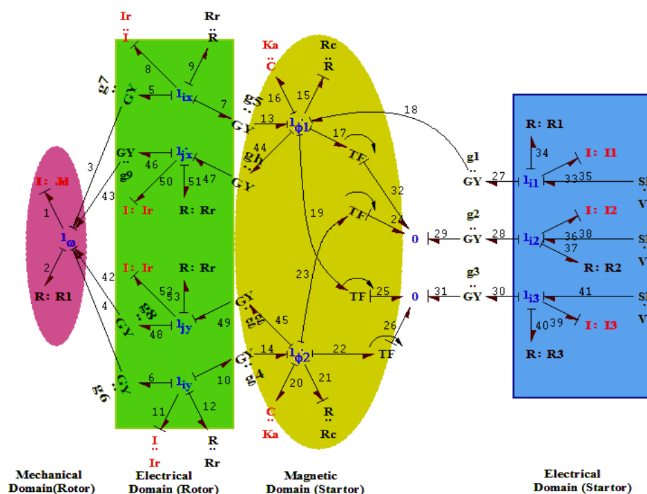
Fig. 6: Bond graph Sub model of three phase four pole induction motor used in Ladle Crane
