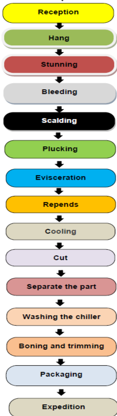
Fig. 1: Flowchart of the turkey leg quarter processing
