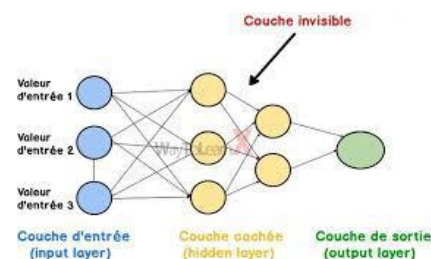
Fig.5: Neural structure
