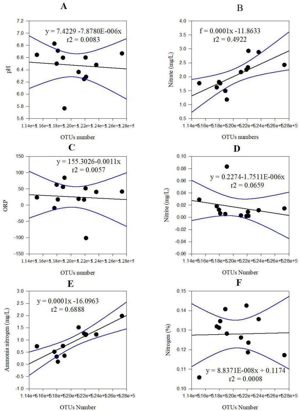
Fig.1: Correlation between pH (A), content of nitrate (B), nitrite (D), amoniactal nitrogen (E), nitrogen (F) and ORP (C) with identified OTU number.
