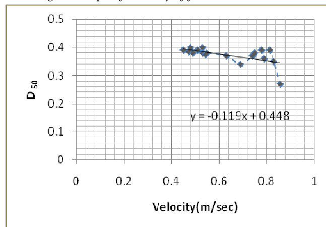
Fig. 4: Graph of D_{50} with Velocity
