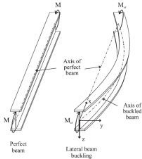
Fig. 4: I- Section Undergoing Lateral Torsional Buckling, Rémi St-Amour, 2016
